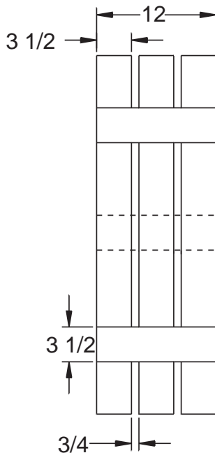
3 Wide Board-N-Batten Spaced Assembly
