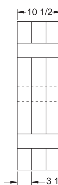
3 Wide Board-N-Batten Joined Assembly
