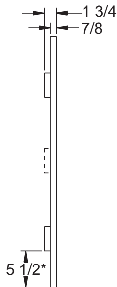
3 Wide Board-N-Batten Spaced Assembly
